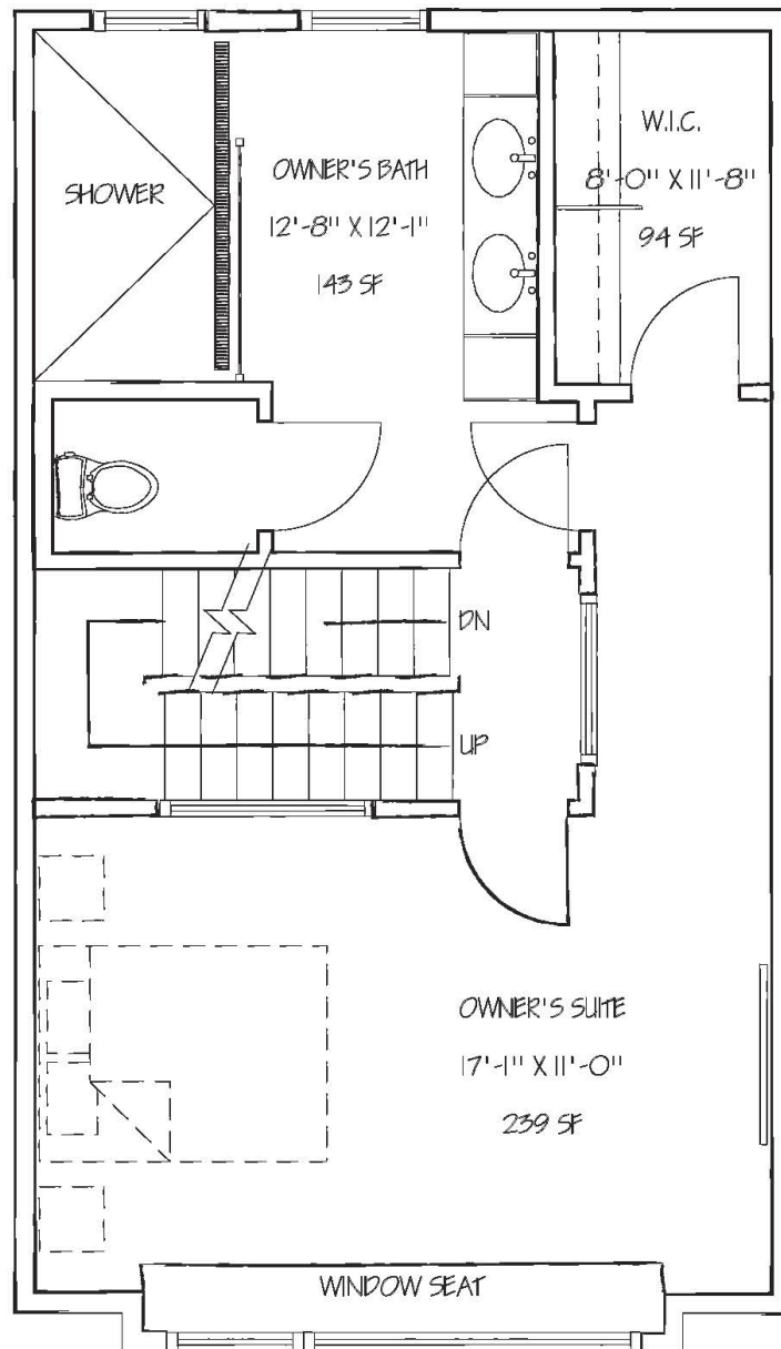
1421 THIRD FLOOR PLAN
