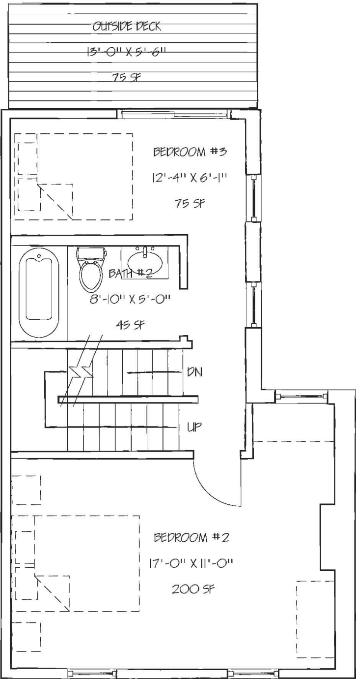
1421 SECOND FLOOR PLAN
