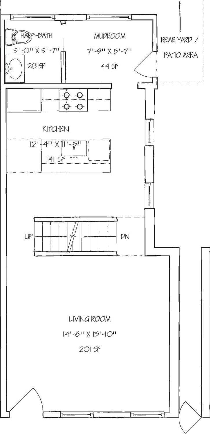
1421 FIRST FLOOR PLAN
