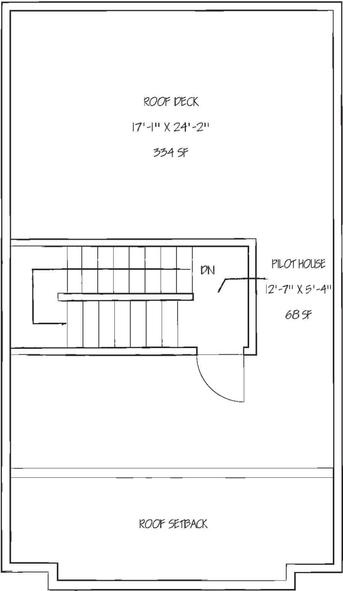
1421 ROOF PLAN
